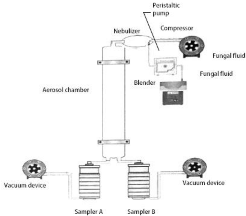
Figure B.2 Bacterial filtration efficiency two-way acquisition test instrumentation diagram
